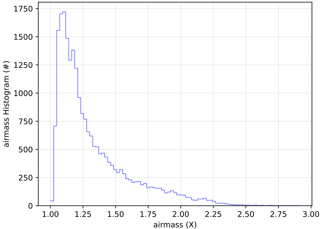
roll_uniform_early_half_mjdp0_v3.4_10yrs Yr 1 g band: airmass Histogram
