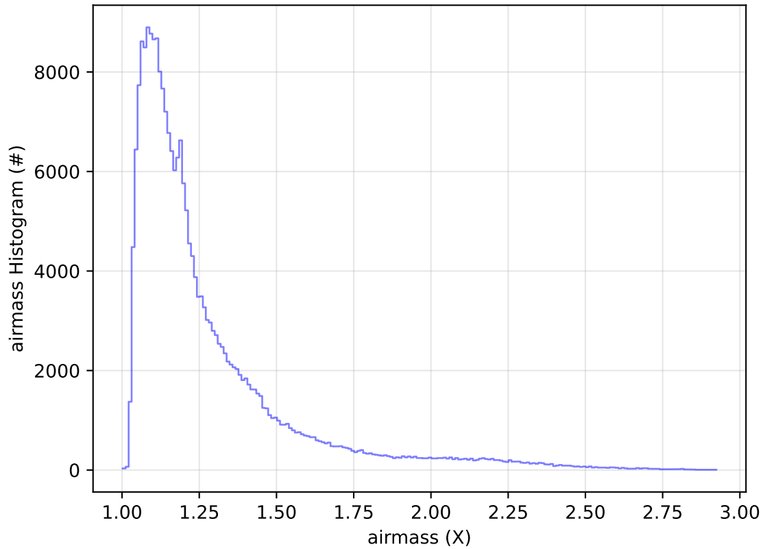
roll_uniform_early_half_mjdp0_v3.4_10yrs Yr 1 all bands: airmass Histogram
