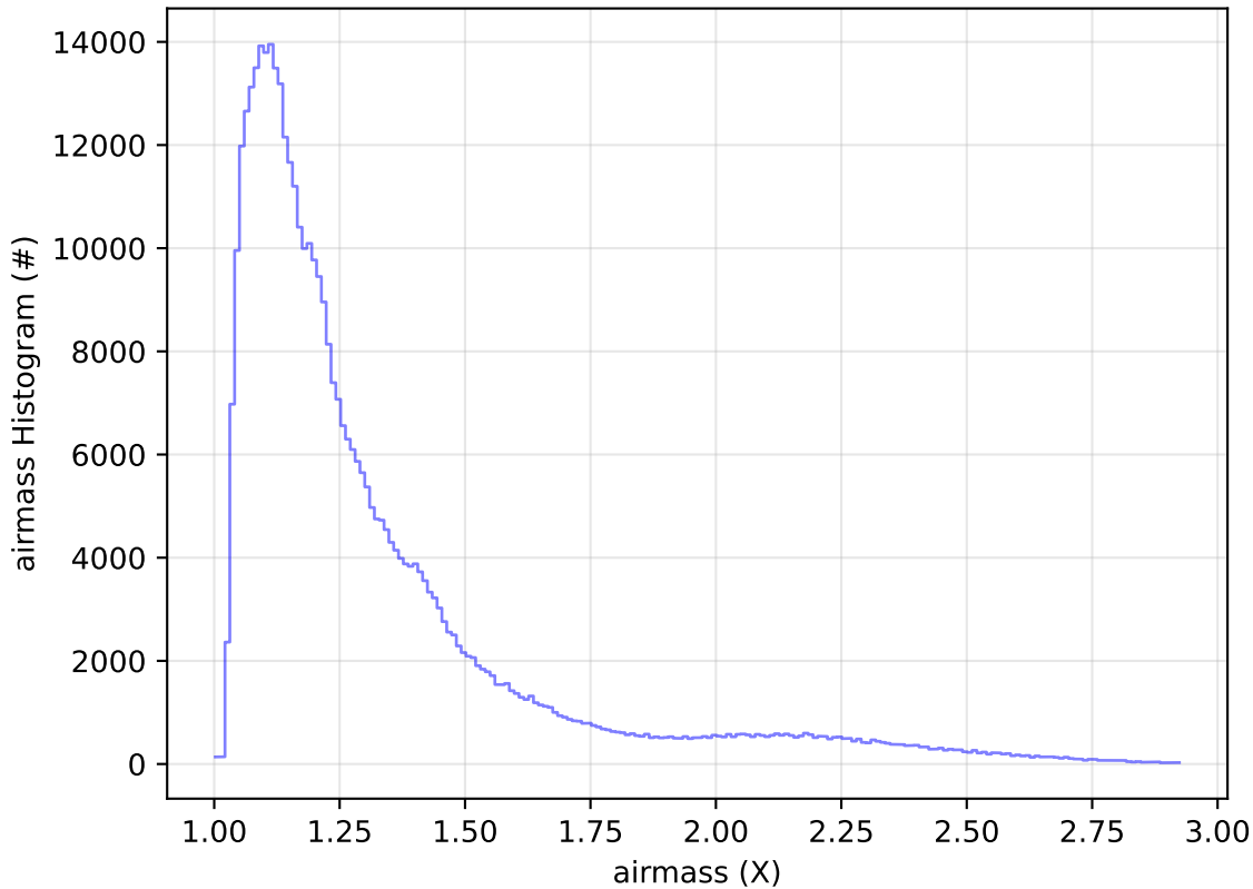
roll_uniform_early_half_mjdp0_v3.4_10yrs WFD z band: airmass Histogram
