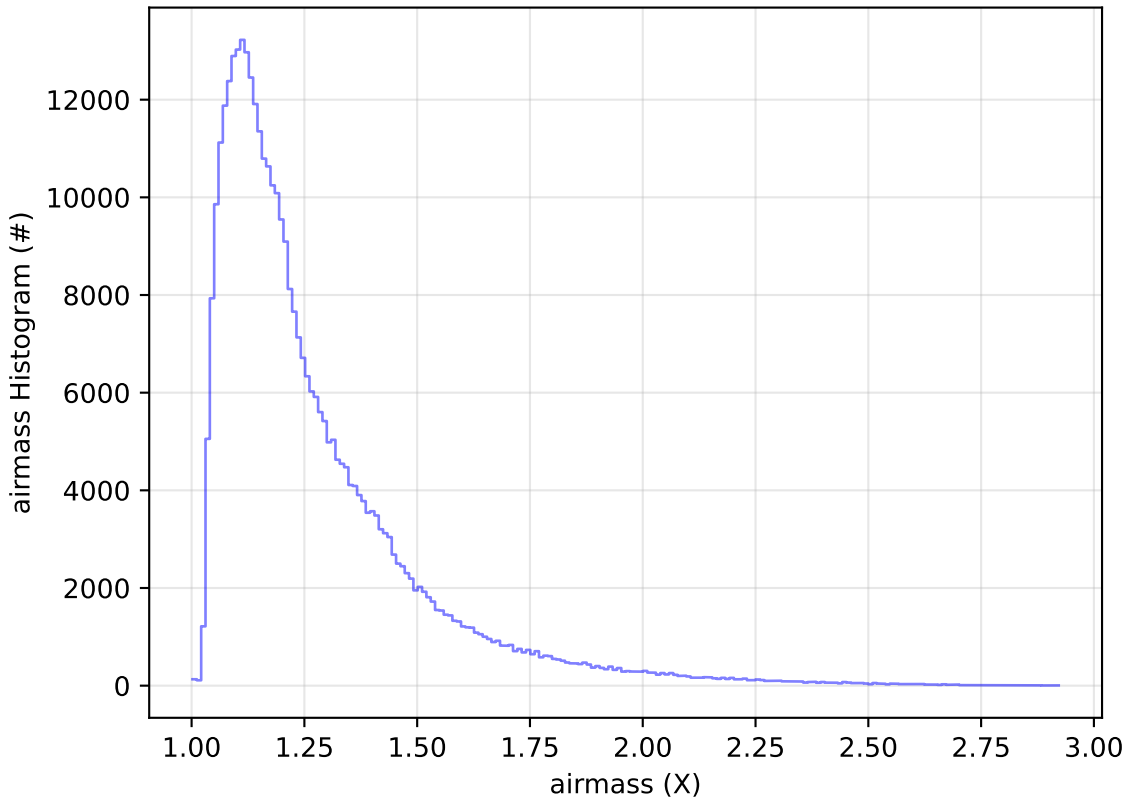
roll_uniform_early_half_mjdp0_v3.4_10yrs WFD y band: airmass Histogram
