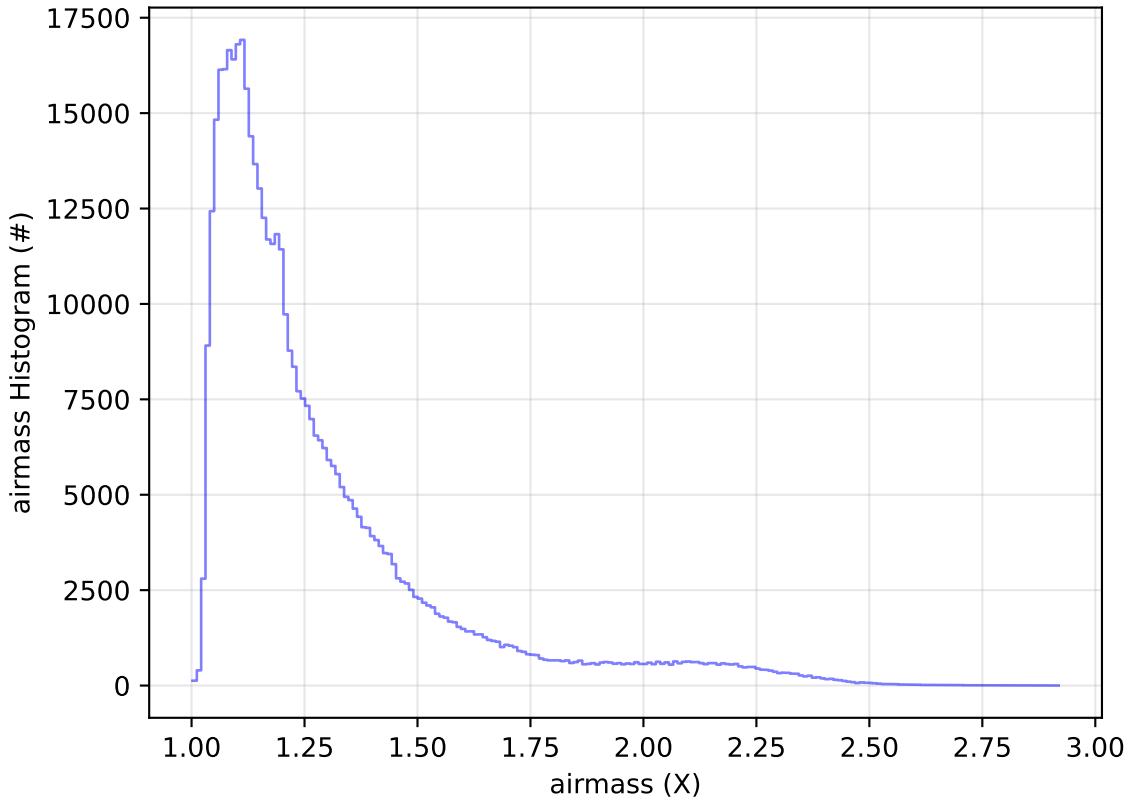
roll_uniform_early_half_mjdp0_v3.4_10yrs WFD r band: airmass Histogram
