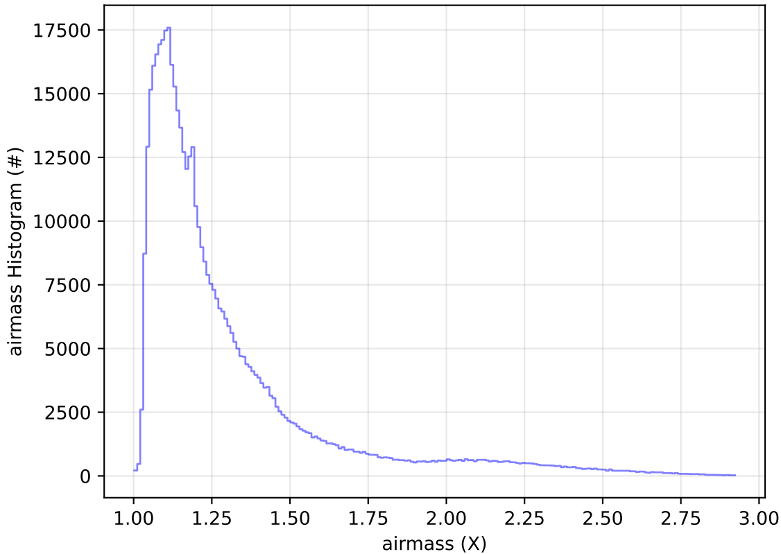
roll_uniform_early_half_mjdp0_v3.4_10yrs WFD i band: airmass Histogram
