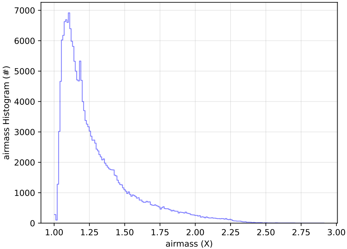
roll_uniform_early_half_mjdp0_v3.4_10yrs WFD g band: airmass Histogram
