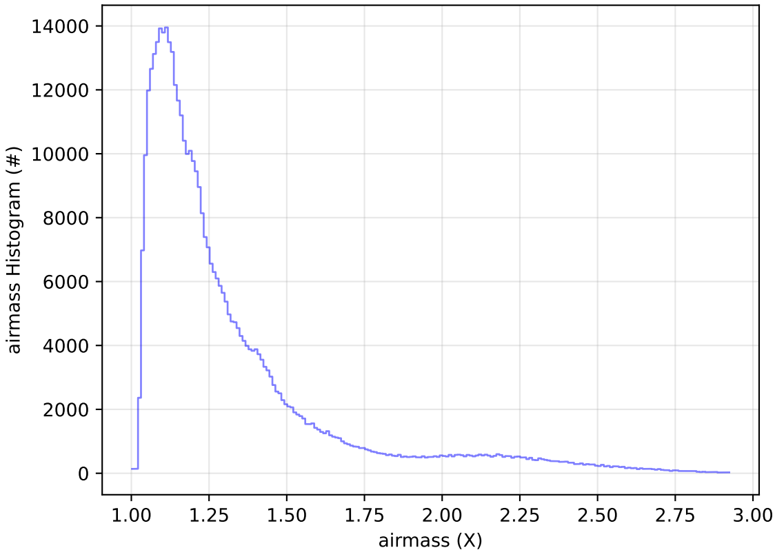
roll_uniform_early_half_mjdp0_v3.4_10yrs All sky z band: airmass Histogram
