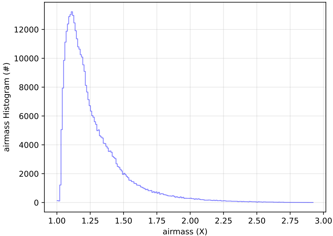
roll_uniform_early_half_mjdp0_v3.4_10yrs All sky y band: airmass Histogram
