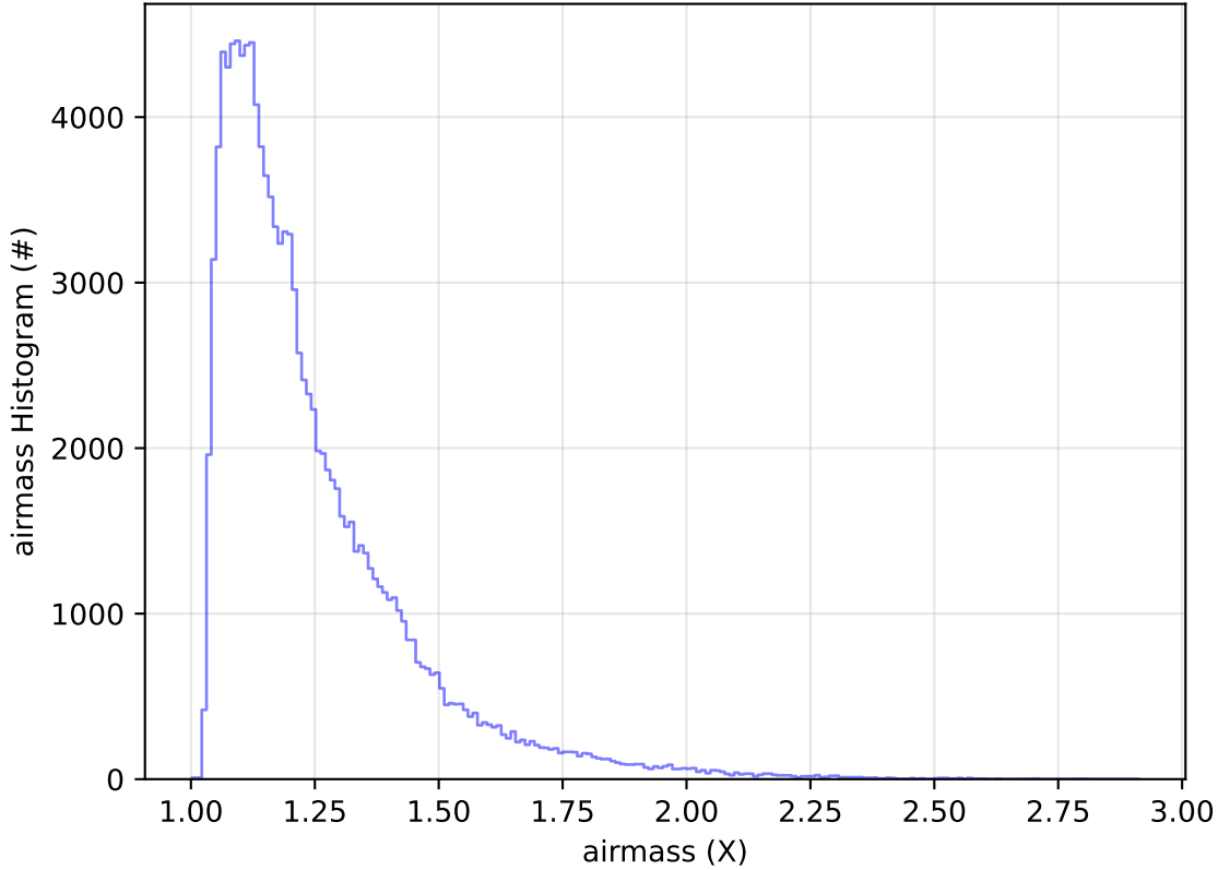
roll_uniform_early_half_mjdp0_v3.4_10yrs All sky u band: airmass Histogram
