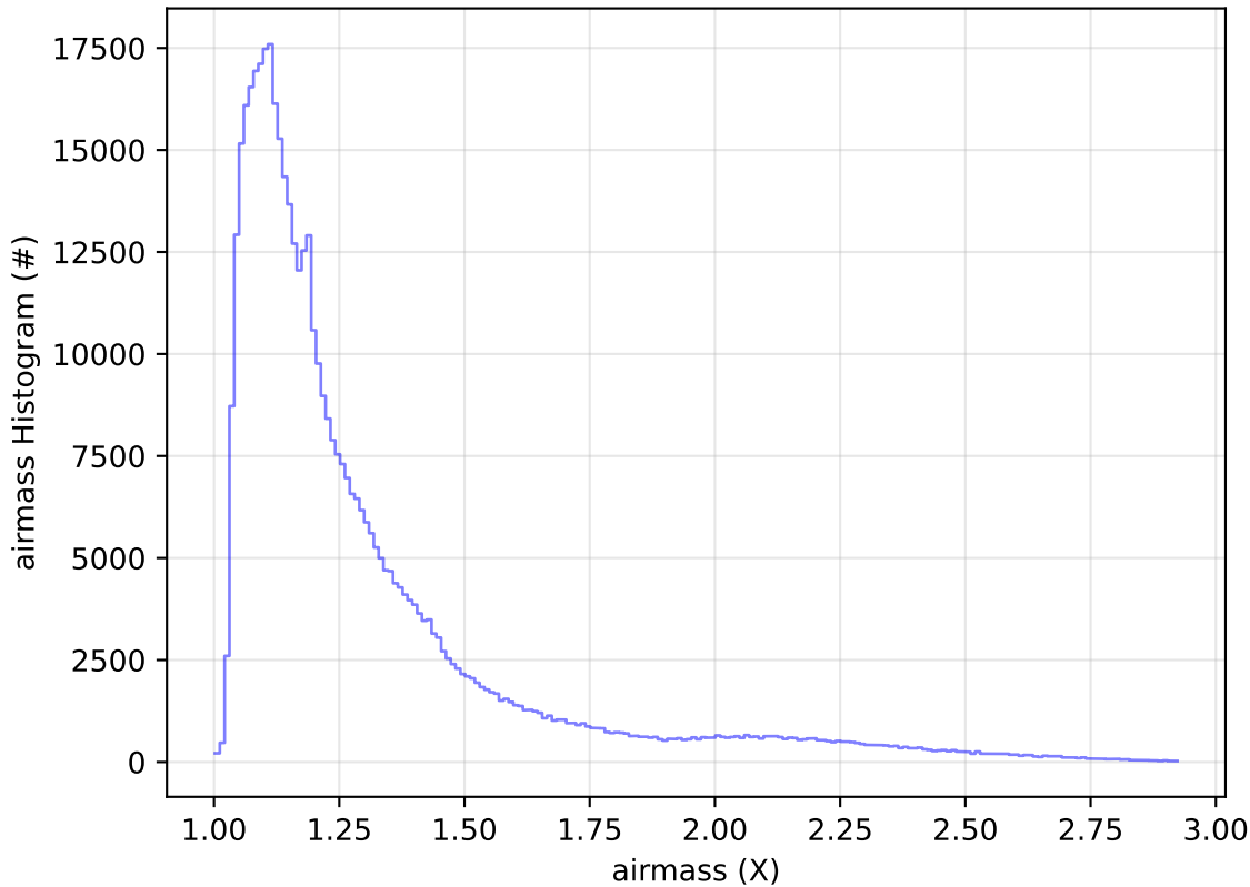
roll_uniform_early_half_mjdp0_v3.4_10yrs All sky i band: airmass Histogram
