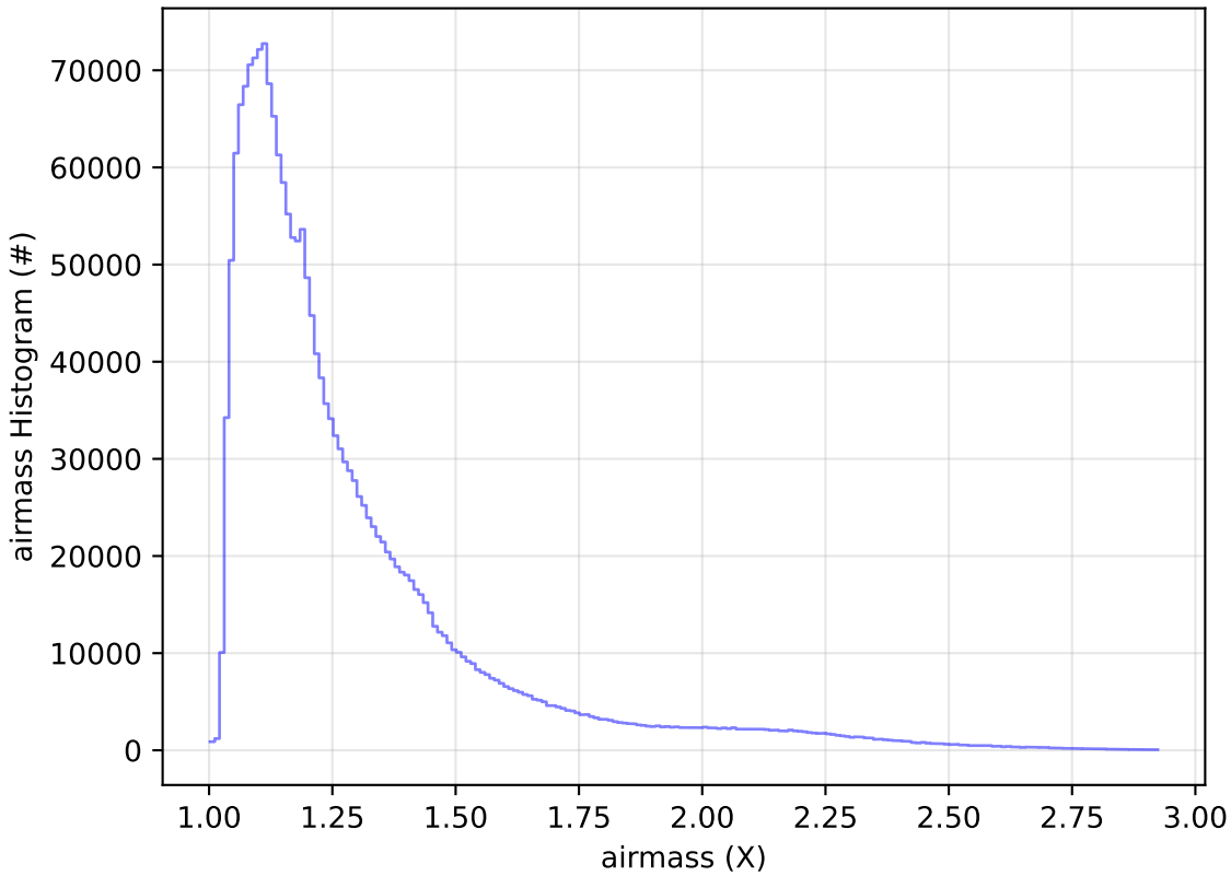
roll_uniform_early_half_mjdp0_v3.4_10yrs All sky all bands: airmass Histogram
