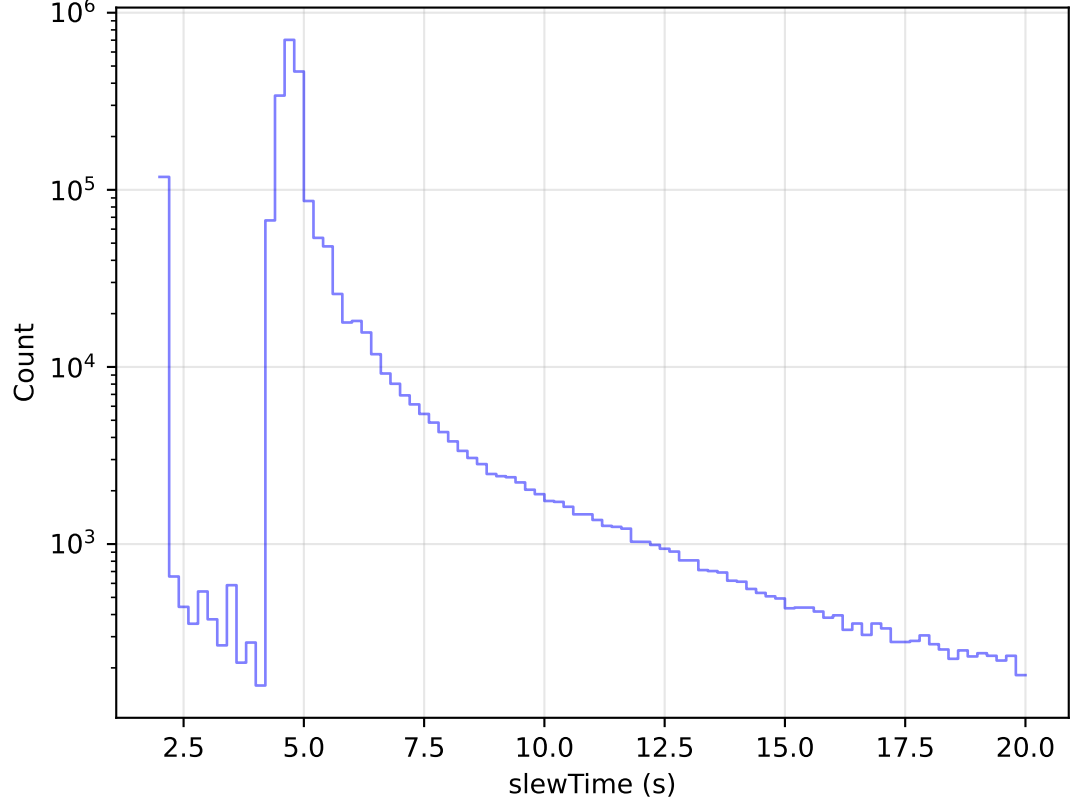
roll_uniform_early_half_mjdp0_v3.4_10yrs All visits: Zoom Slew Time Histogram
