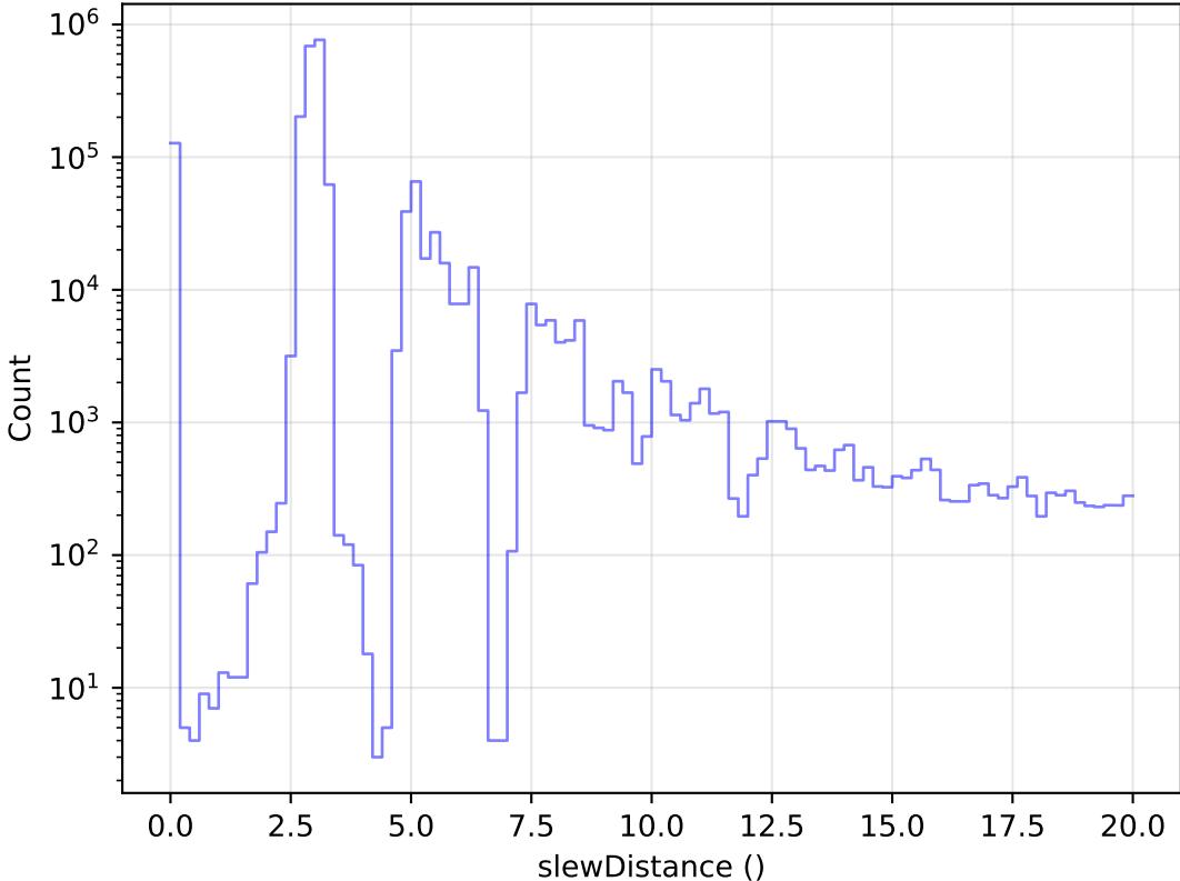
roll_uniform_early_half_mjdp0_v3.4_10yrs All visits: Zoom Slew Distance Histogram
