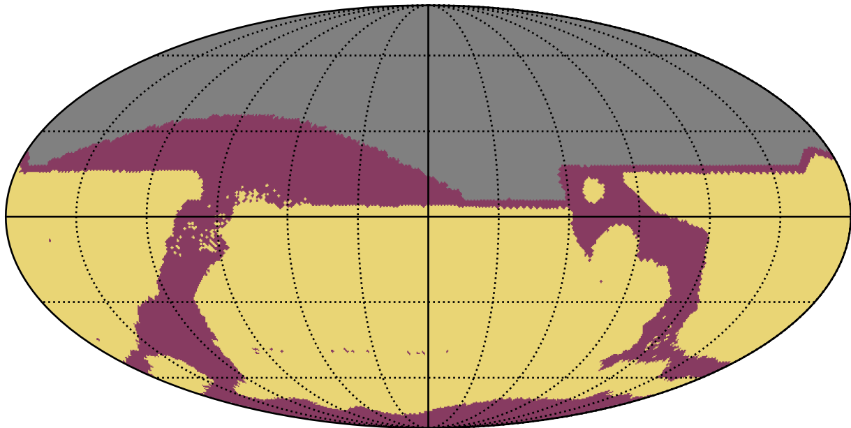
roll_uniform_early_half_mjdp0_v3.4_10yrs All sky: RapidRevisits
