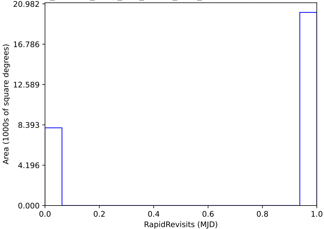
roll_uniform_early_half_mjdp0_v3.4_10yrs All sky: RapidRevisits
