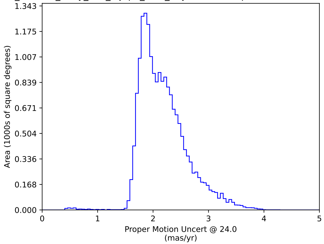
roll_uniform_early_half_mjdp0_v3.4_10yrs WFD: Proper Motion Uncert @ 24.0
