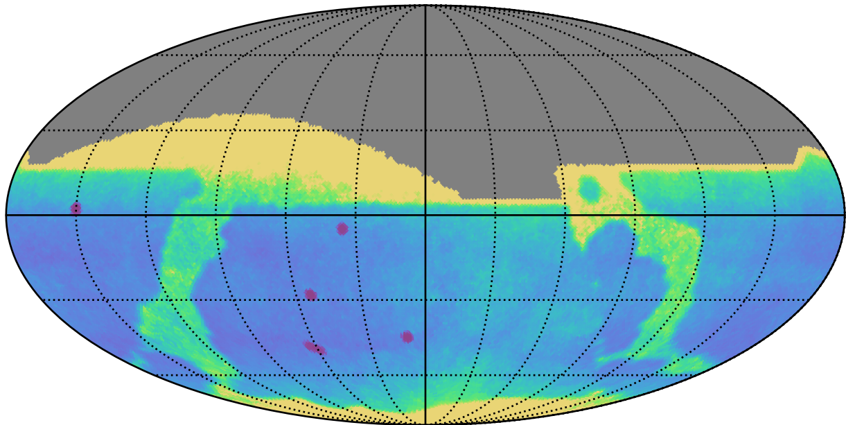
roll_uniform_early_half_mjdp0_v3.4_10yrs All sky: Proper Motion Uncert @ 24.0
