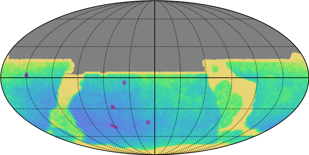
roll_uniform_early_half_mjdp0_v3.4_10yrs All sky y band only: Parallax Uncert @ 21.3
