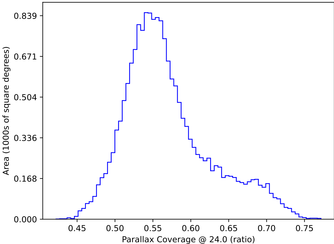
roll_uniform_early_half_mjdp0_v3.4_10yrs WFD: Parallax Coverage @ 24.0
