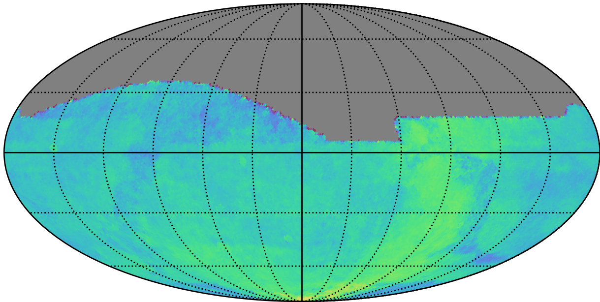
roll_uniform_early_half_mjdp0_v3.4_10yrs All sky: Parallax Coverage @ 24.0
