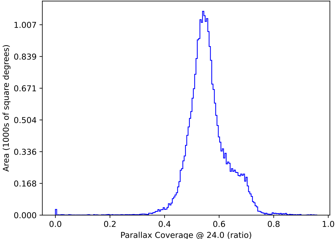
roll_uniform_early_half_mjdp0_v3.4_10yrs All sky: Parallax Coverage @ 24.0
