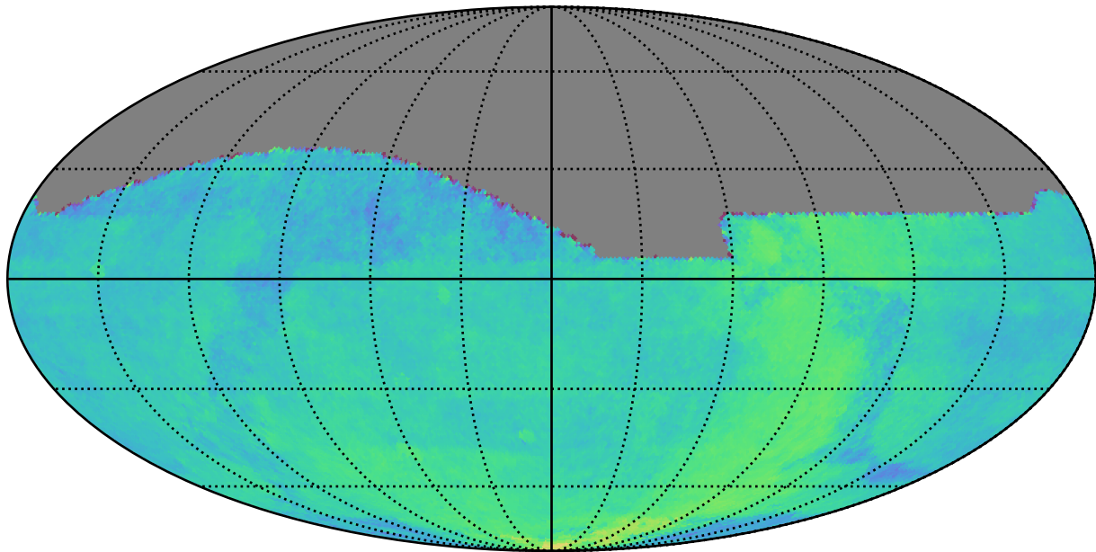
roll_uniform_early_half_mjdp0_v3.4_10yrs All sky: Parallax Coverage @ 22.4
