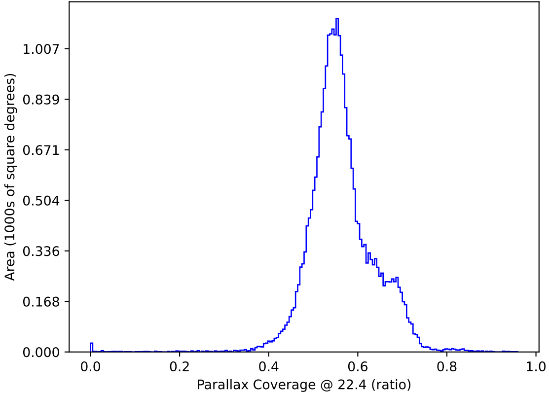
roll_uniform_early_half_mjdp0_v3.4_10yrs All sky: Parallax Coverage @ 22.4
