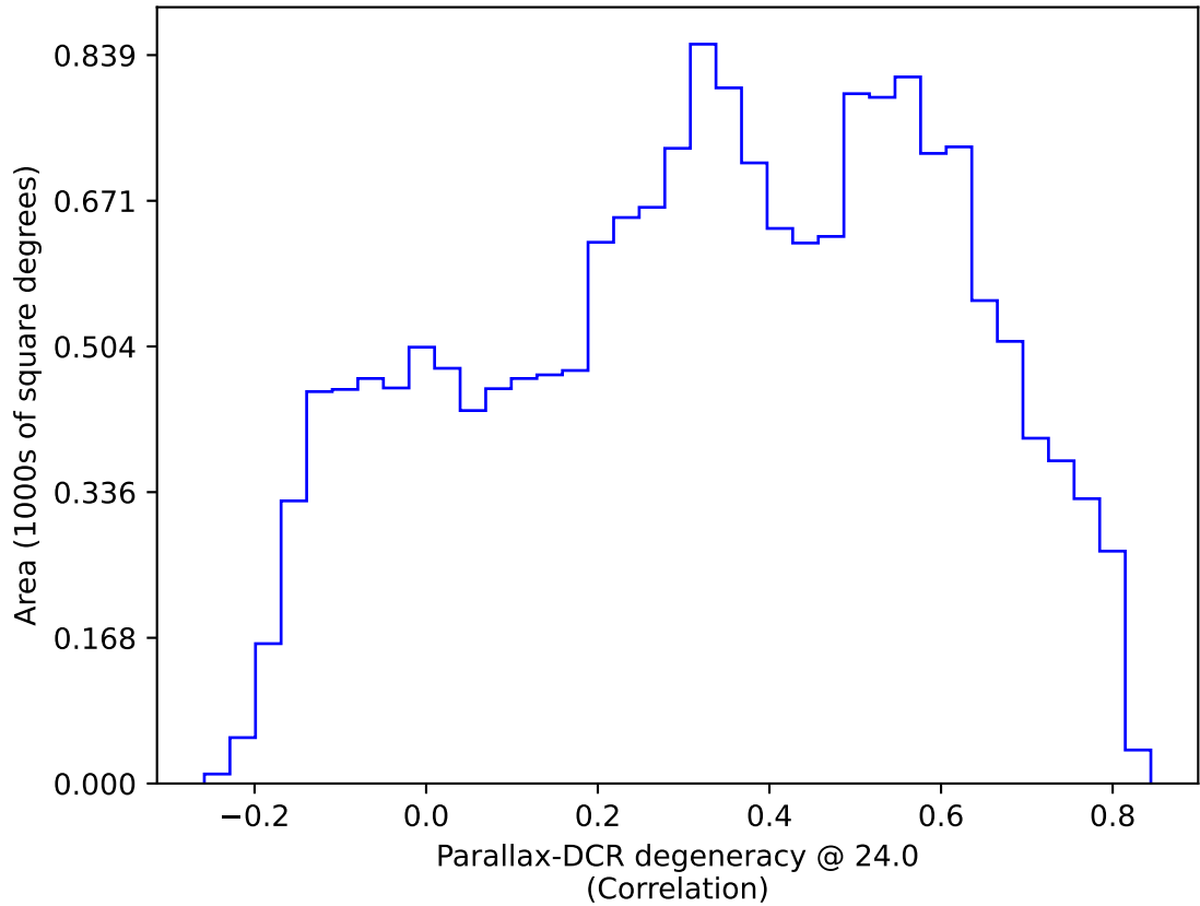
roll_uniform_early_half_mjdp0_v3.4_10yrs WFD: Parallax-DCR degeneracy @ 24.0
