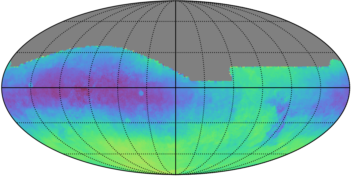
roll_uniform_early_half_mjdp0_v3.4_10yrs All sky: Parallax-DCR degeneracy @ 24.0
