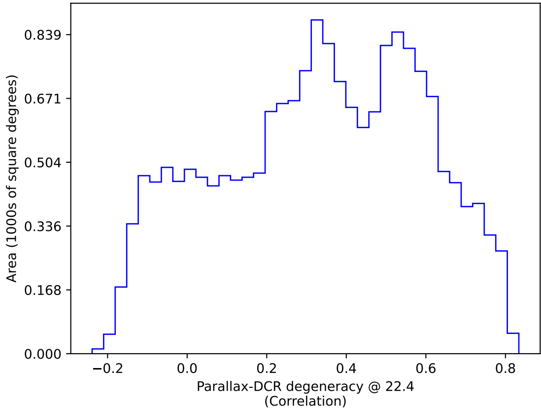
roll_uniform_early_half_mjdp0_v3.4_10yrs WFD: Parallax-DCR degeneracy @ 22.4
