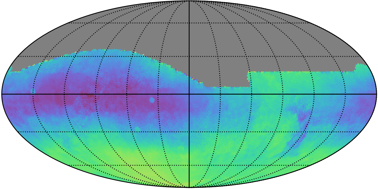
roll_uniform_early_half_mjdp0_v3.4_10yrs All sky: Parallax-DCR degeneracy @ 22.4
