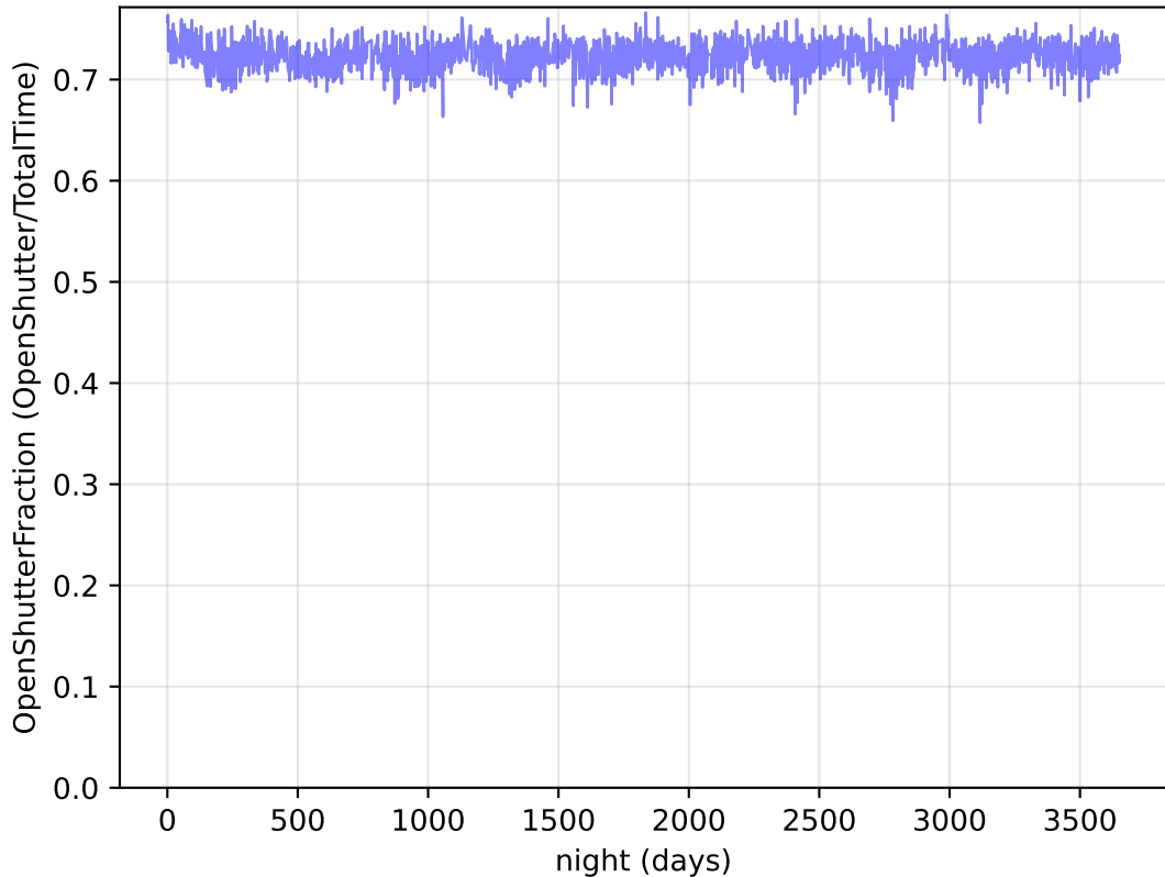
roll_uniform_early_half_mjdp0_v3.4_10yrs Per night: OpenShutterFraction
