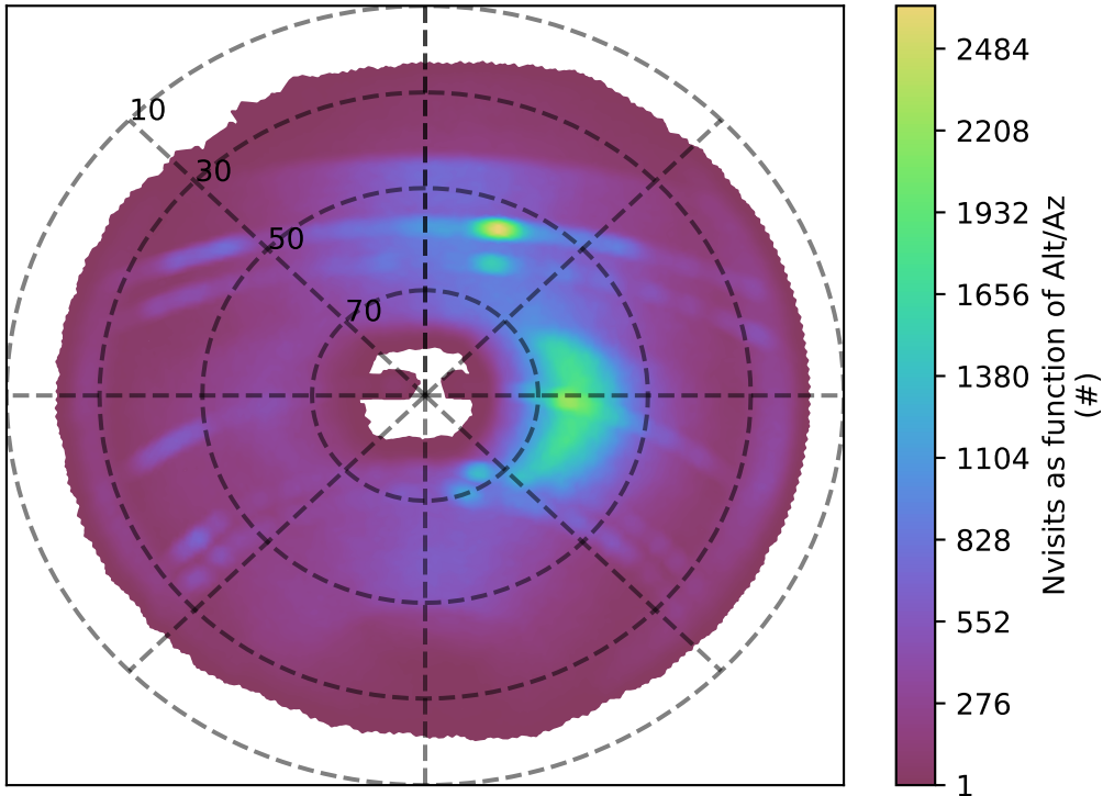
roll_uniform_early_half_mjdp0_v3.4_10yrs z band: Nvisits as function of Alt/Az
