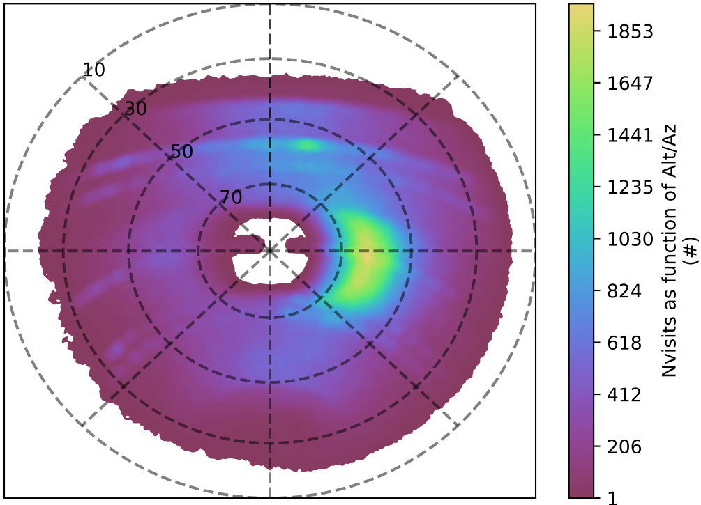
roll_uniform_early_half_mjdp0_v3.4_10yrs y band: Nvisits as function of Alt/Az
