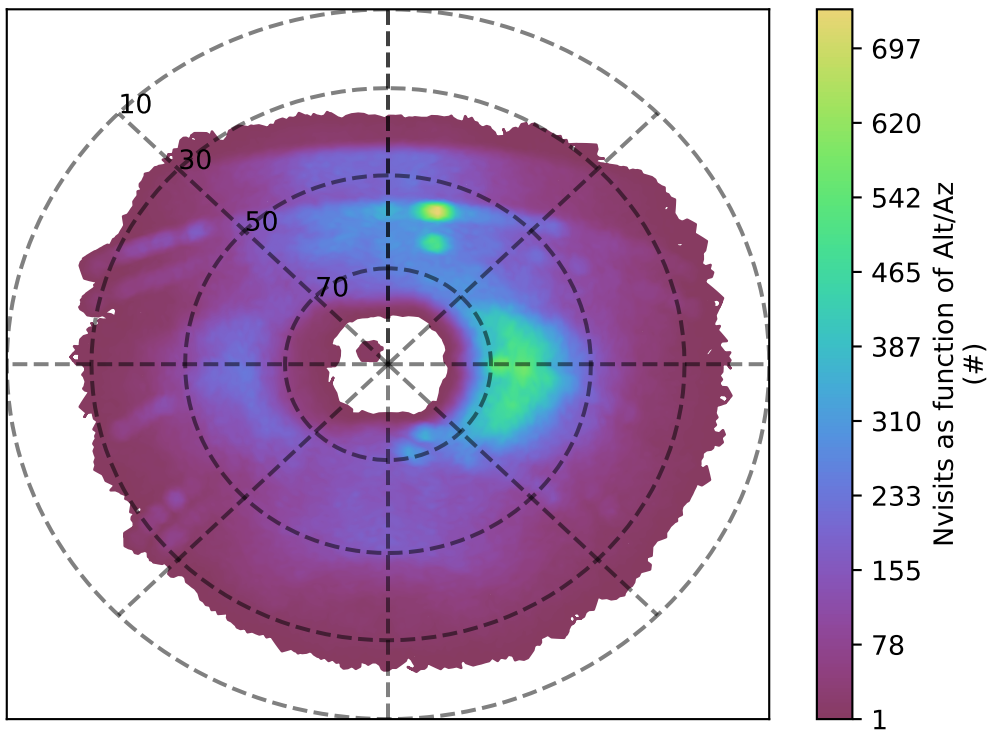
roll_uniform_early_half_mjdp0_v3.4_10yrs u band: Nvisits as function of Alt/Az
