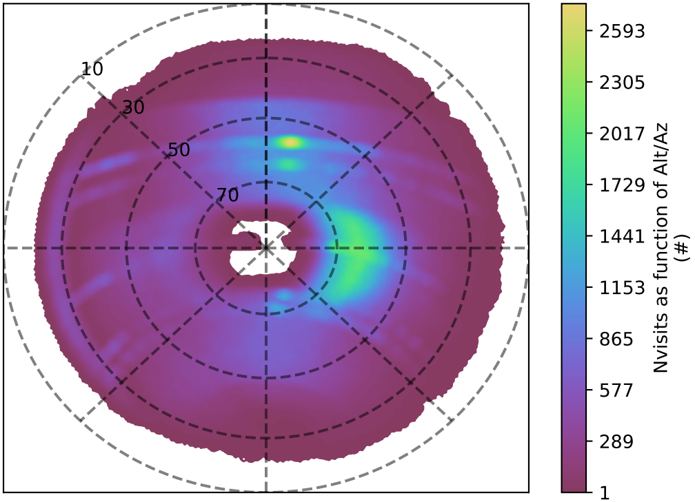
roll_uniform_early_half_mjdp0_v3.4_10yrs r band: Nvisits as function of Alt/Az
