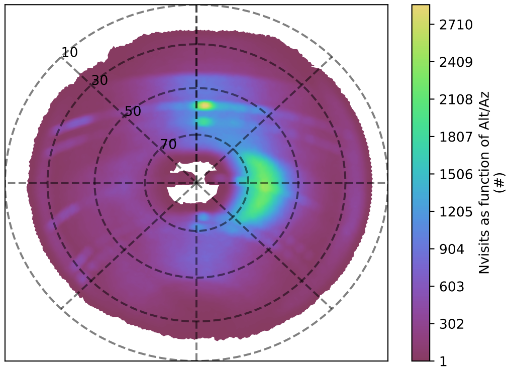
roll_uniform_early_half_mjdp0_v3.4_10yrs i band: Nvisits as function of Alt/Az
