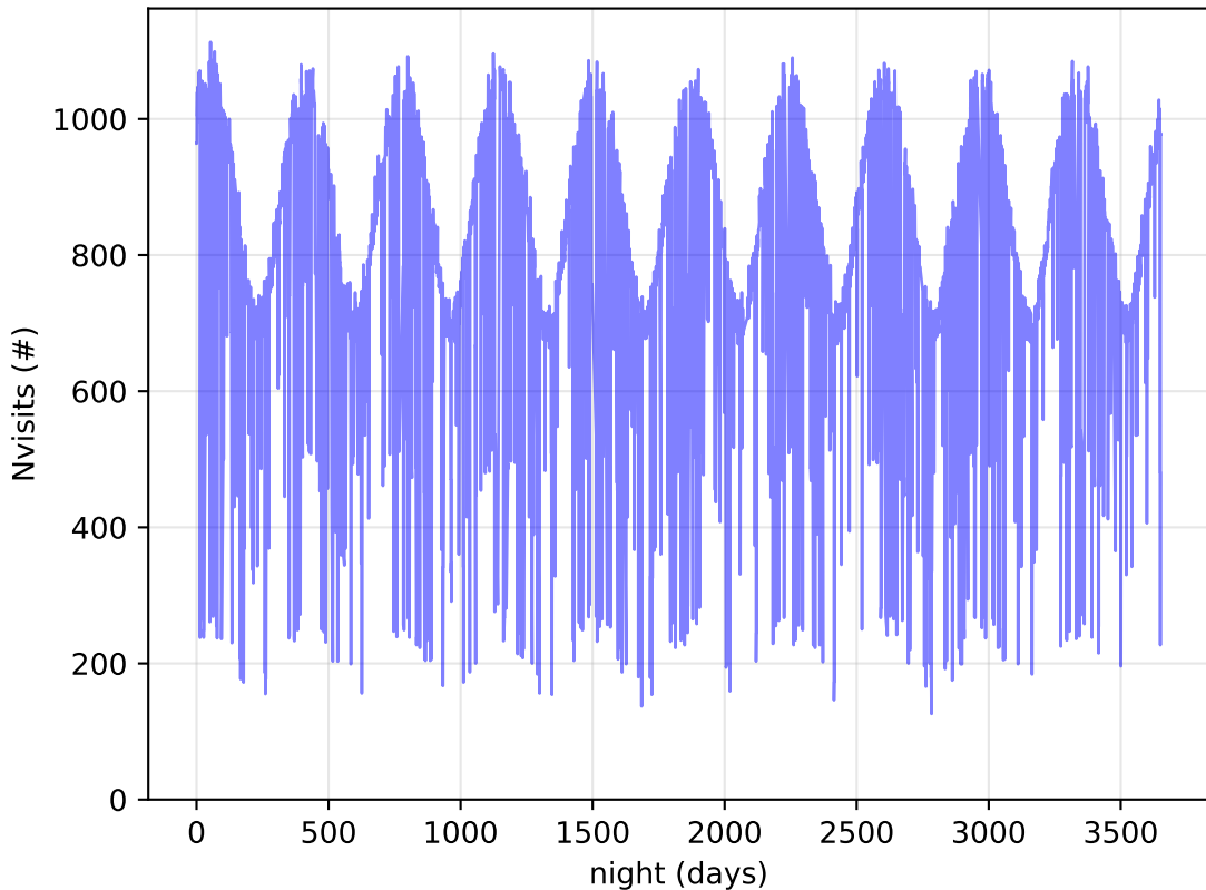
roll_uniform_early_half_mjdp0_v3.4_10yrs All visits: Nvisits
