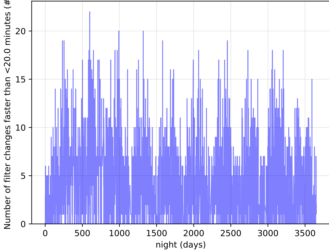
roll_uniform_early_half_mjdp0_v3.4_10yrs Per Night: Number of filter changes faster than <20.0 minutes
