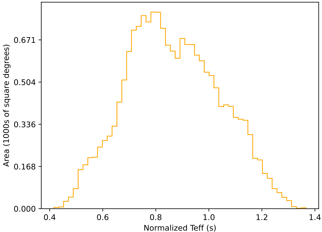
roll_uniform_early_half_mjdp0_v3.4_10yrs WFD r band: Normalized Teff
