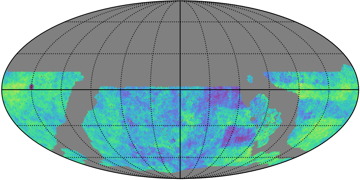
roll_uniform_early_half_mjdp0_v3.4_10yrs WFD: Normalized Proper Motion Uncert @ 24.0
