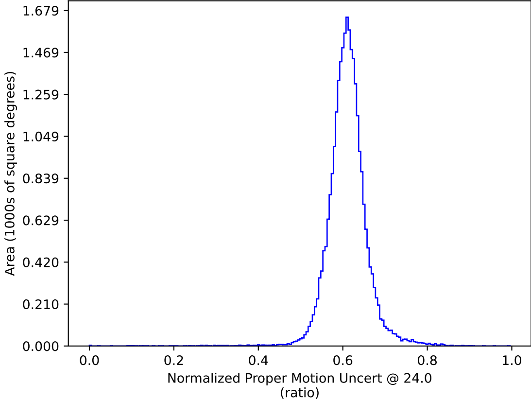
roll_uniform_early_half_mjdp0_v3.4_10yrs All sky: Normalized Proper Motion Uncert @ 24.0
