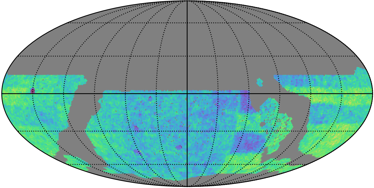
roll_uniform_early_half_mjdp0_v3.4_10yrs WFD: Normalized Proper Motion Uncert @ 20.5
