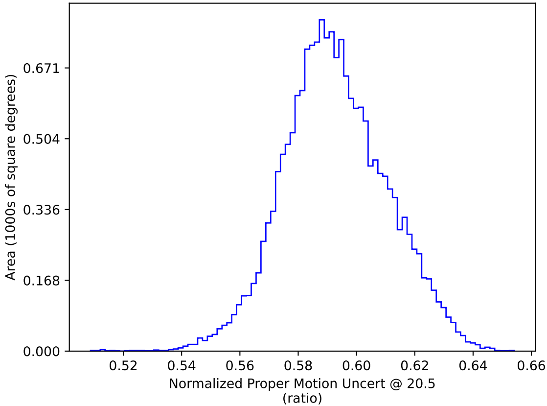
roll_uniform_early_half_mjdp0_v3.4_10yrs WFD: Normalized Proper Motion Uncert @ 20.5
