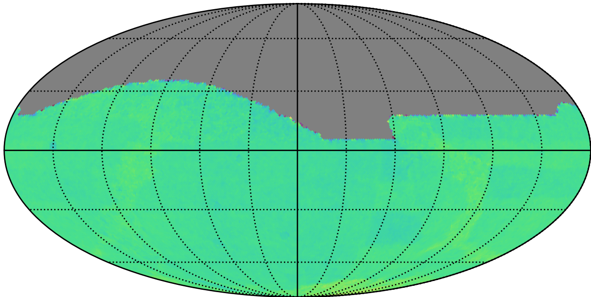
roll_uniform_early_half_mjdp0_v3.4_10yrs All sky: Normalized Proper Motion Uncert @ 20.5
