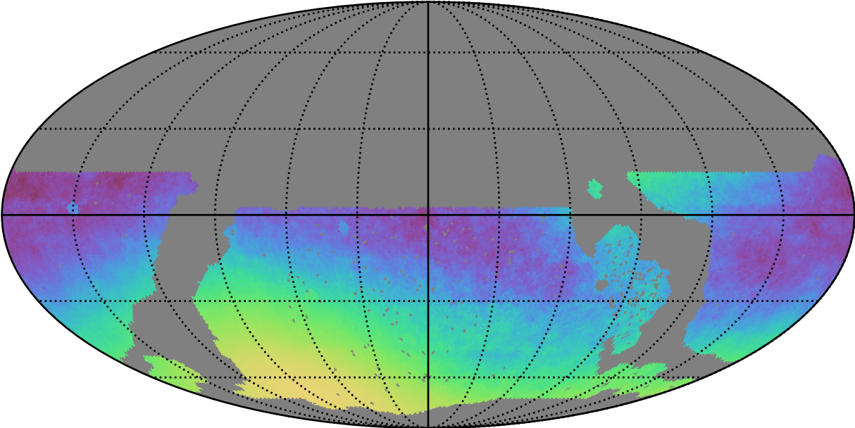
roll_uniform_early_half_mjdp0_v3.4_10yrs WFD: Normalized Parallax Uncert @ 24.0
