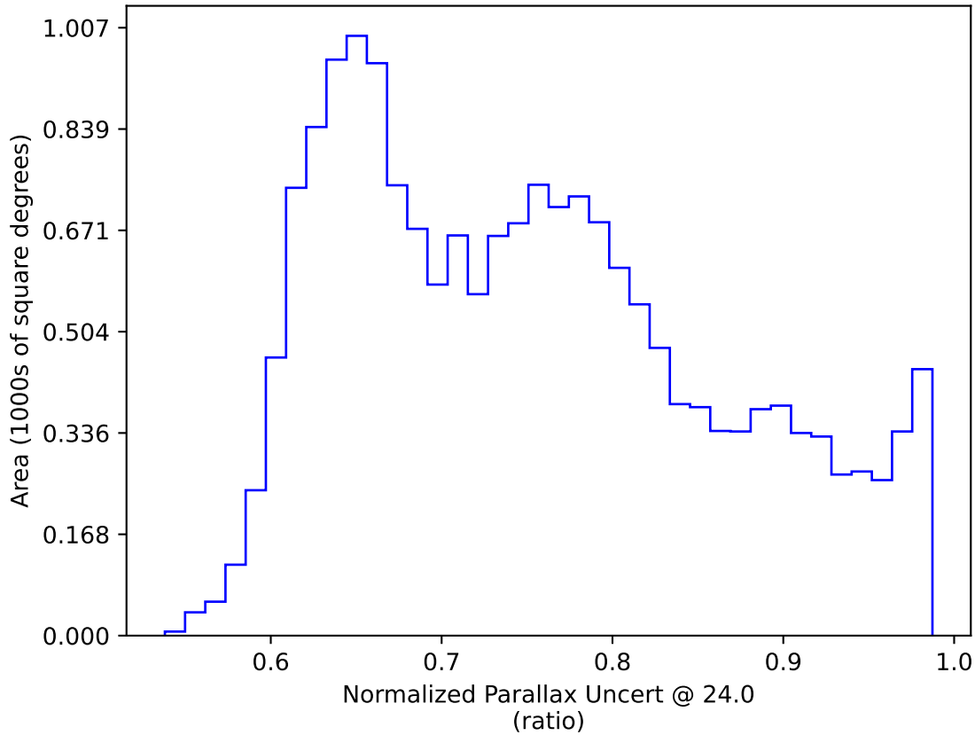
roll_uniform_early_half_mjdp0_v3.4_10yrs WFD: Normalized Parallax Uncert @ 24.0
