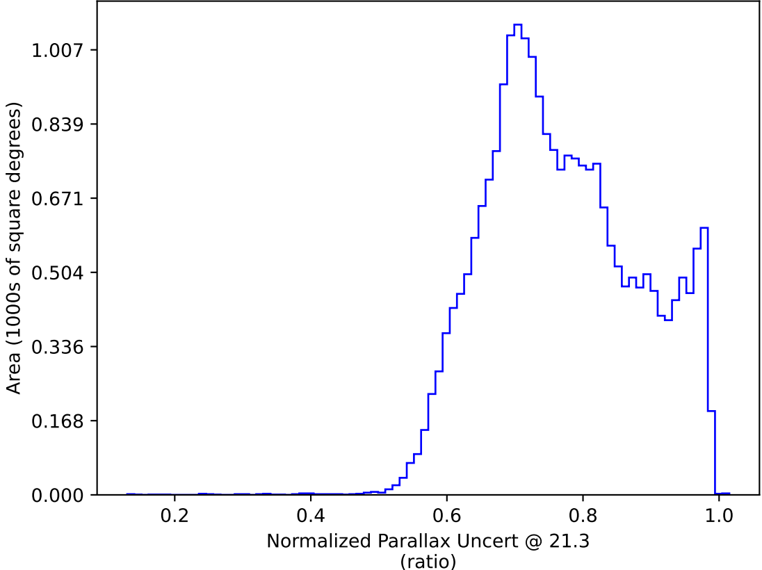
roll_uniform_early_half_mjdp0_v3.4_10yrs All sky y band only: Normalized Parallax Uncert @ 21.3
