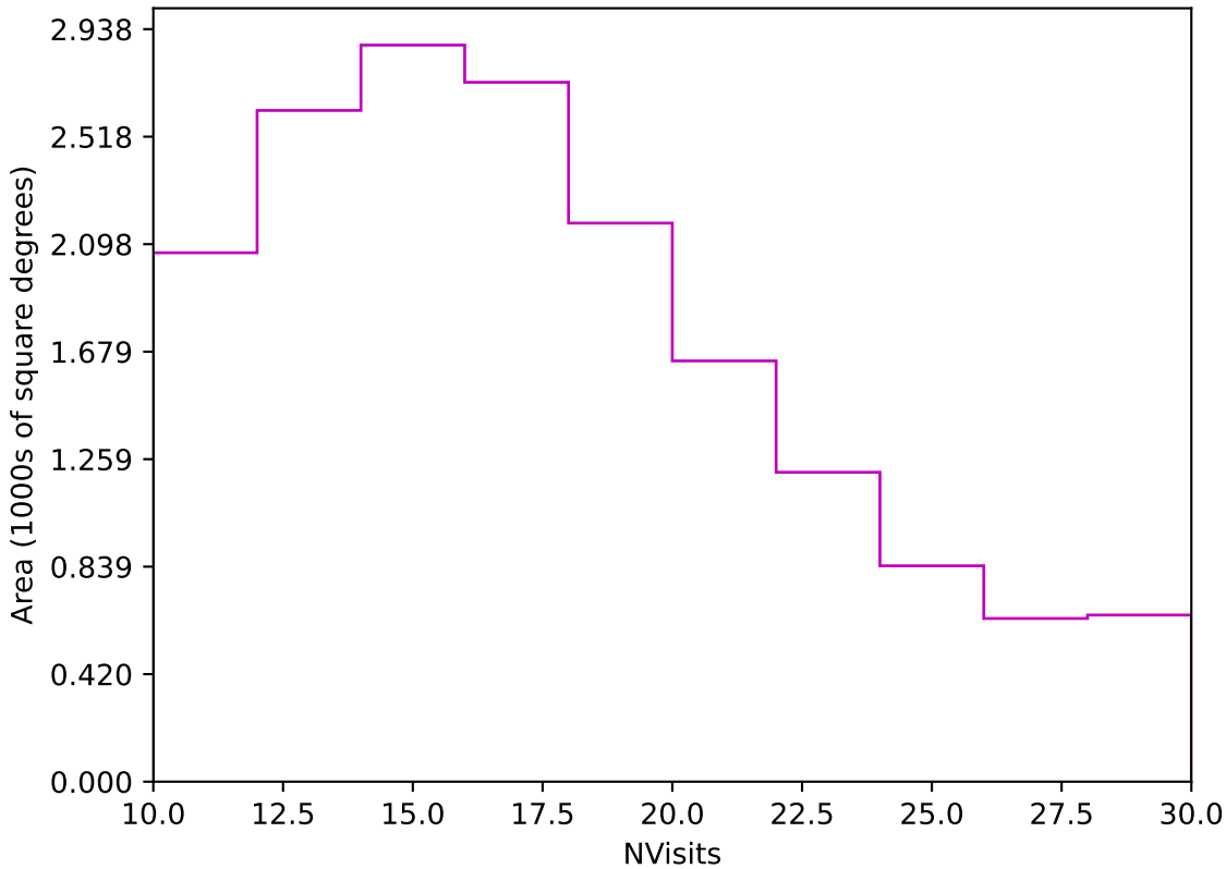
roll_uniform_early_half_mjdp0_v3.4_10yrs Yr 3-4 z band: NVisits
