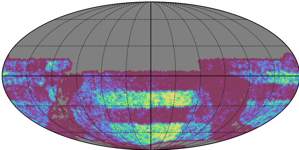
roll_uniform_early_half_mjdp0_v3.4_10yrs Yr 3-4 y band: NVisits
