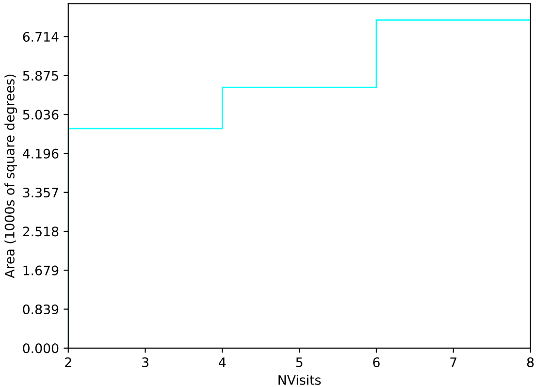
roll_uniform_early_half_mjdp0_v3.4_10yrs Yr 3-4 u band: NVisits
