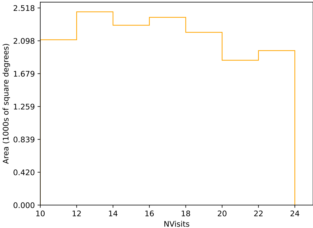
roll_uniform_early_half_mjdp0_v3.4_10yrs Yr 3-4 r band: NVisits
