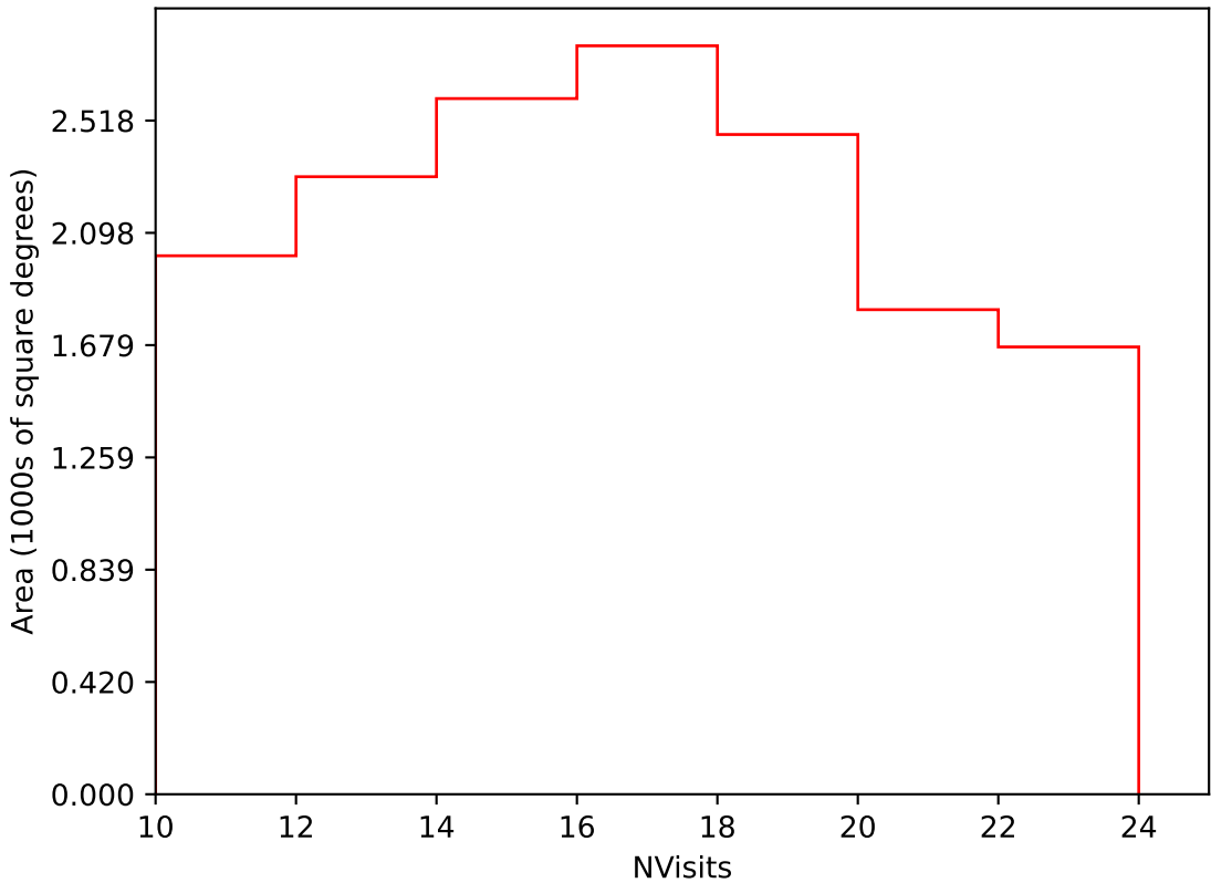
roll_uniform_early_half_mjdp0_v3.4_10yrs Yr 3-4 i band: NVisits
